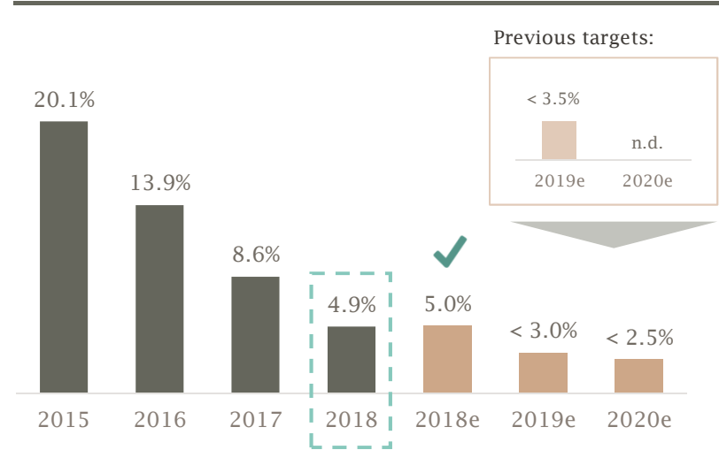
NPL ratio
